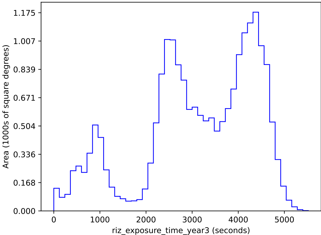
too_5_1v3.4_10yrs gri band non-DD: riz_exposure_time_year3
