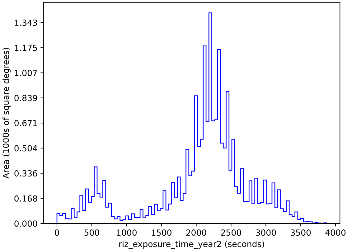
too_5_1v3.4_10yrs gri band non-DD: riz_exposure_time_year2
