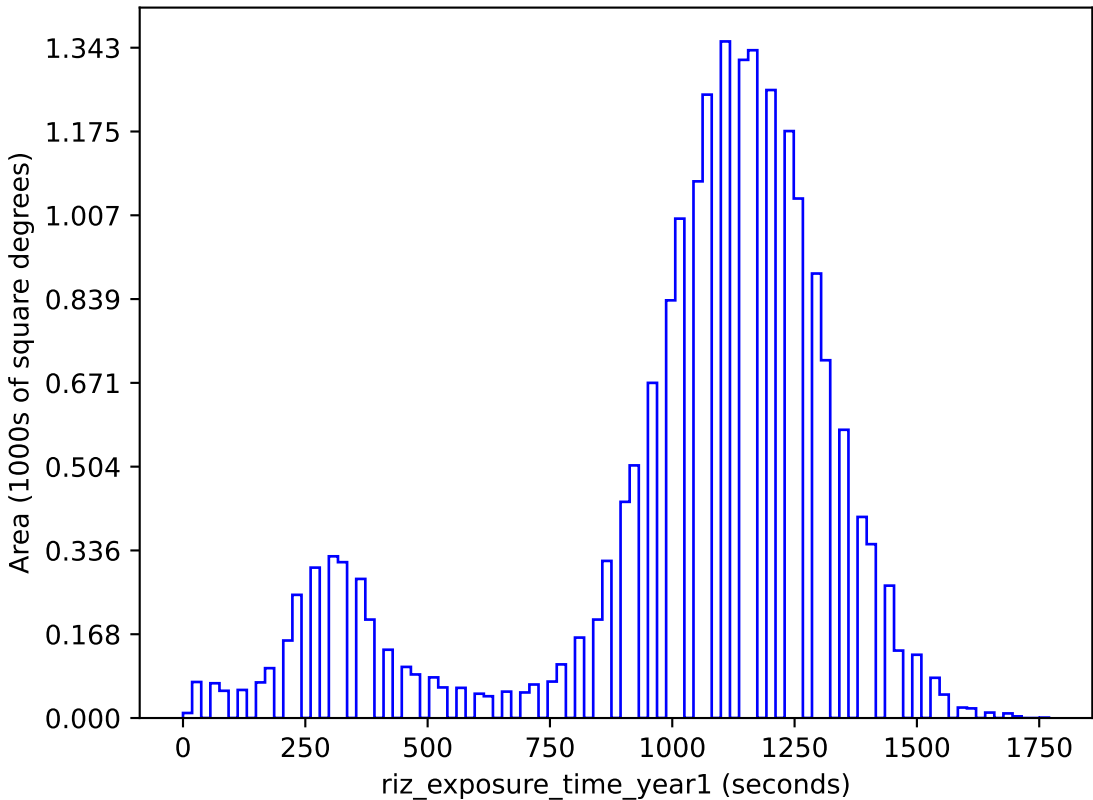
too_5_1v3.4_10yrs gri band non-DD: riz_exposure_time_year1
