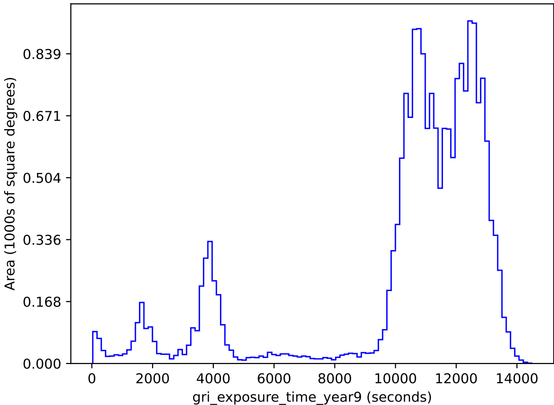
too_5_1v3.4_10yrs gri band non-DD: gri_exposure_time_year9
