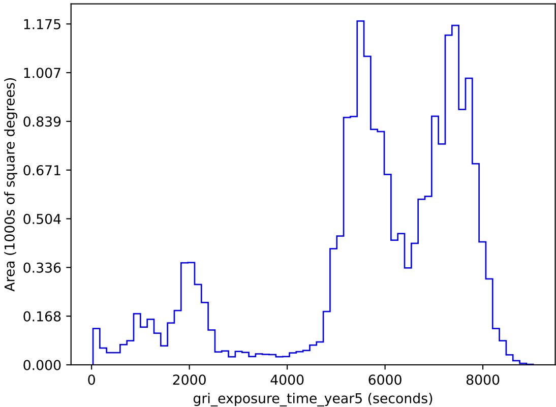
too_5_1v3.4_10yrs gri band non-DD: gri_exposure_time_year5
