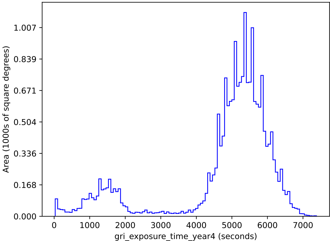
too_5_1v3.4_10yrs gri band non-DD: gri_exposure_time_year4
