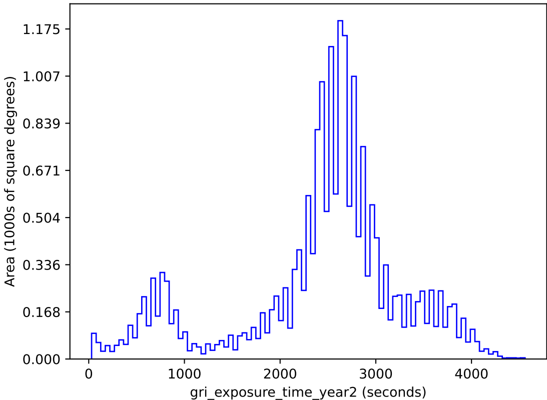
too_5_1v3.4_10yrs gri band non-DD: gri_exposure_time_year2
