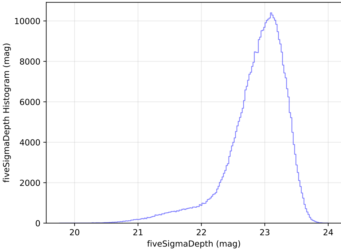
too_5_1v3.4_10yrs z: fiveSigmaDepth Histogram
