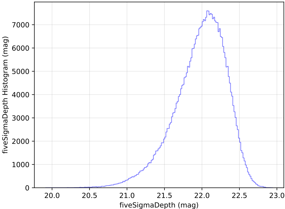
too_5_1v3.4_10yrs y: fiveSigmaDepth Histogram
