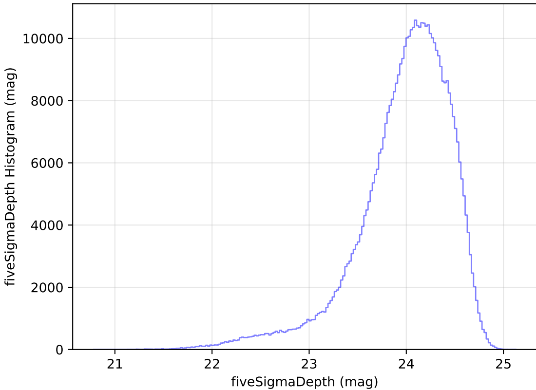
too_5_1v3.4_10yrs r: fiveSigmaDepth Histogram
