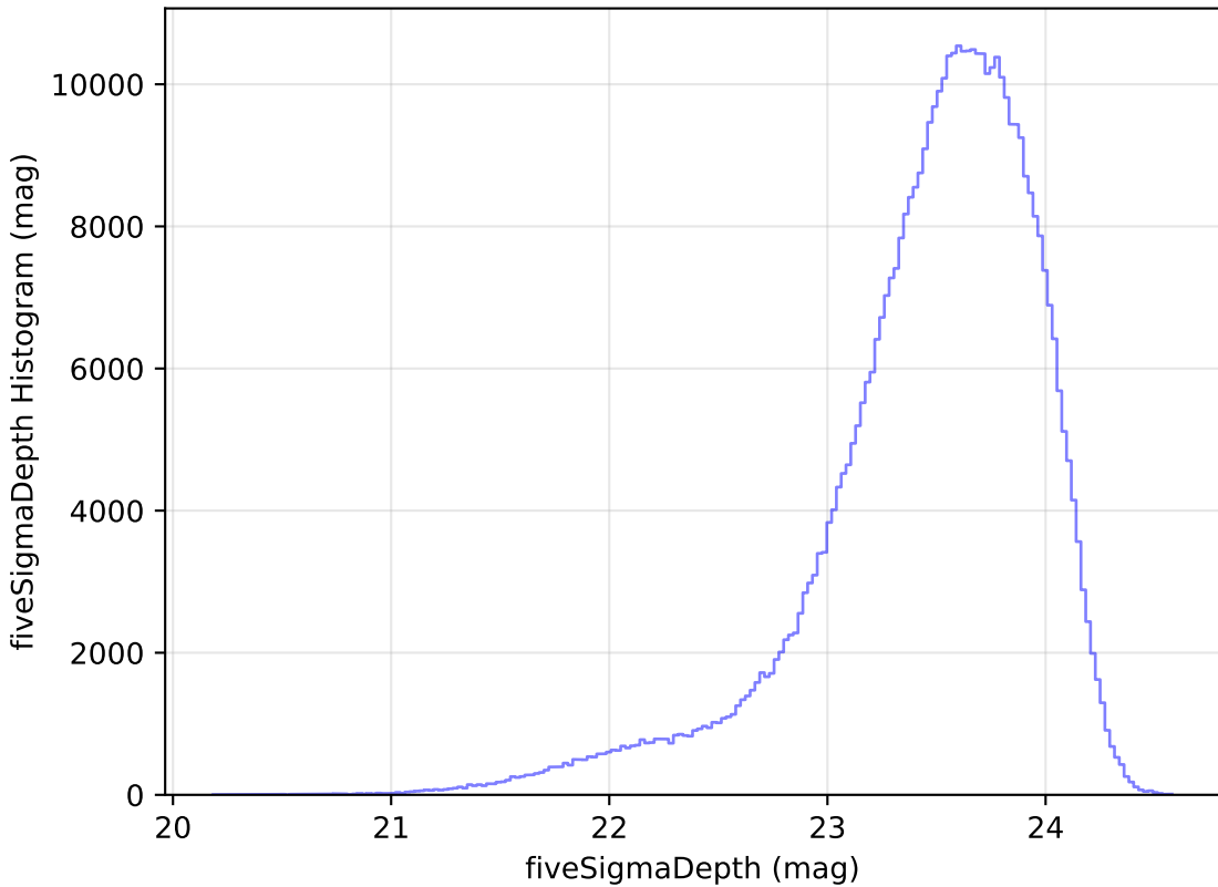
too_5_1v3.4_10yrs i: fiveSigmaDepth Histogram
