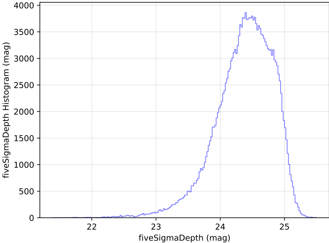
too_5_1v3.4_10yrs g: fiveSigmaDepth Histogram
