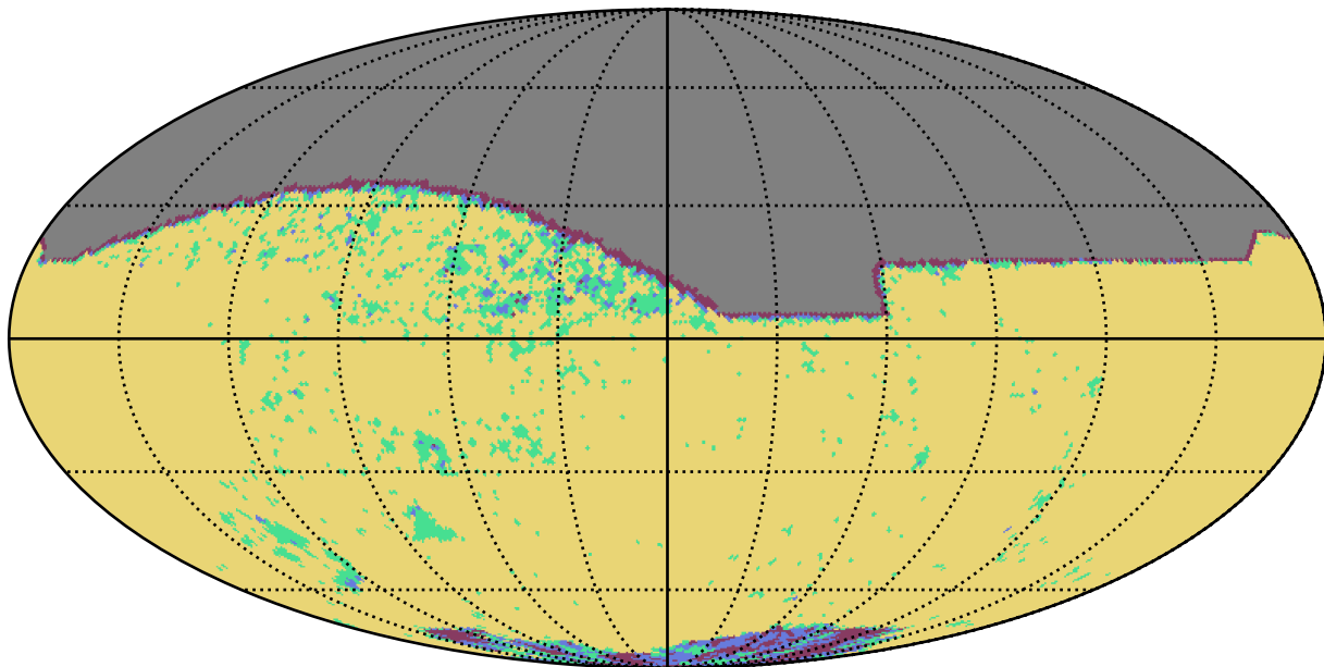
too_5_1v3.4_10yrs z band: YearCoverage night
