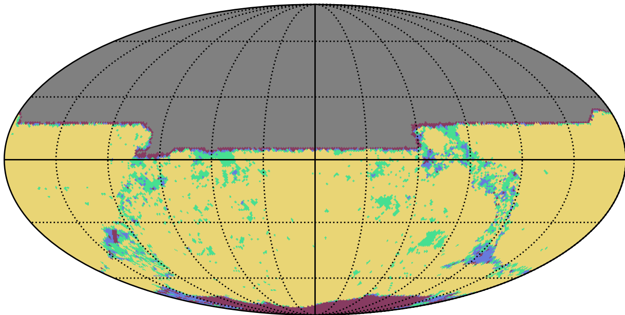
too_5_1v3.4_10yrs y band: YearCoverage night
