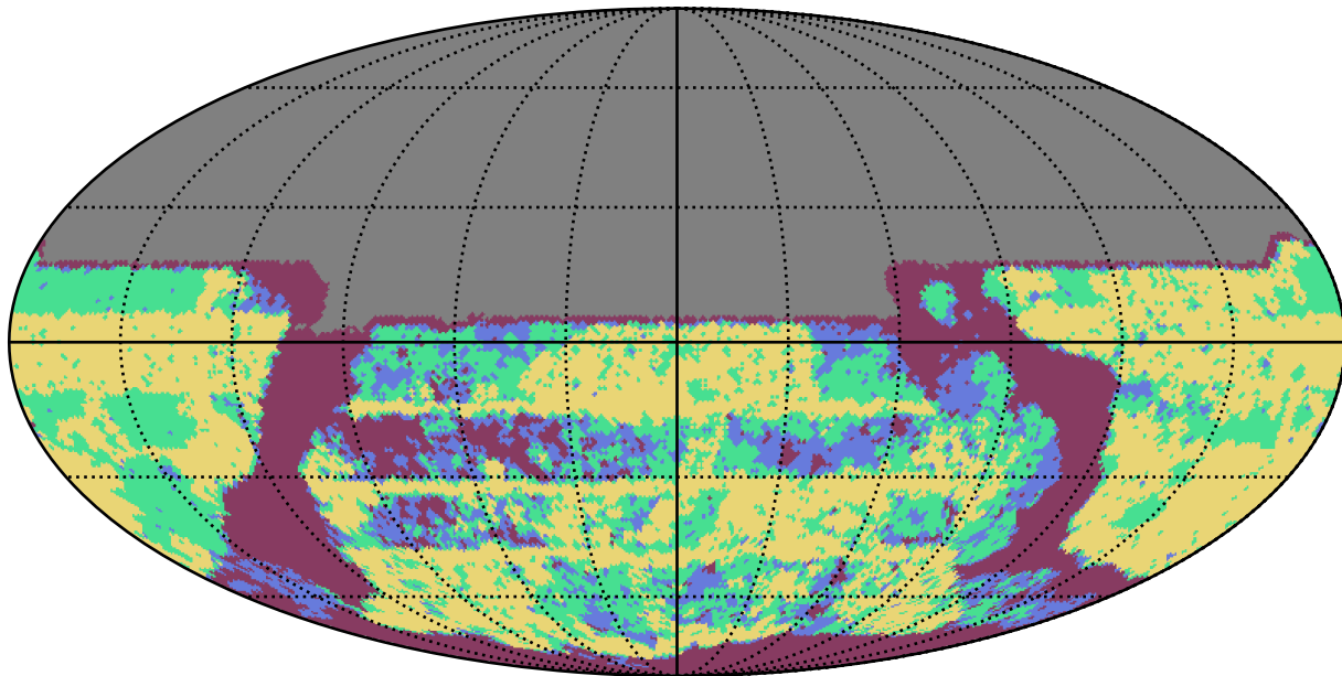
too_5_1v3.4_10yrs u band: YearCoverage night
