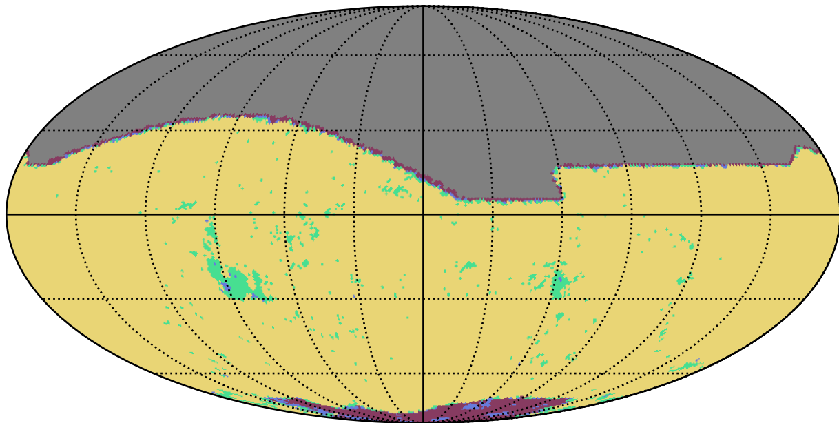
too_5_1v3.4_10yrs r band: YearCoverage night
