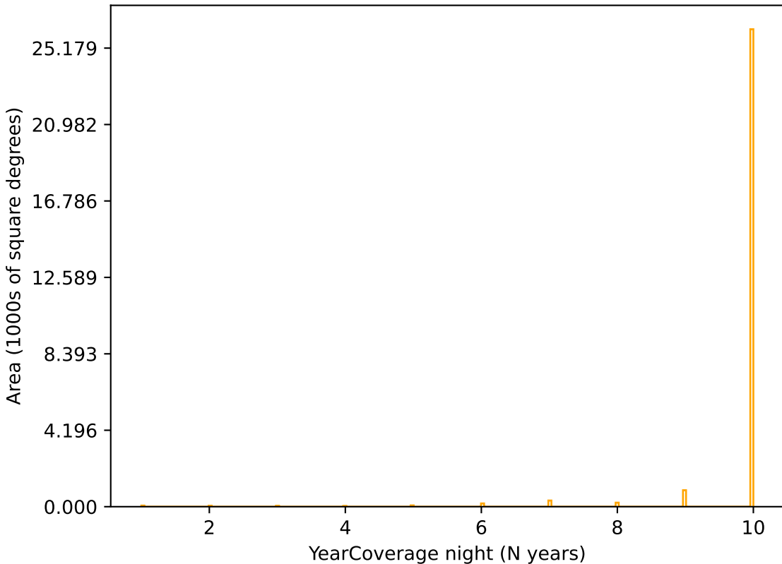
too_5_1v3.4_10yrs r band: YearCoverage night
