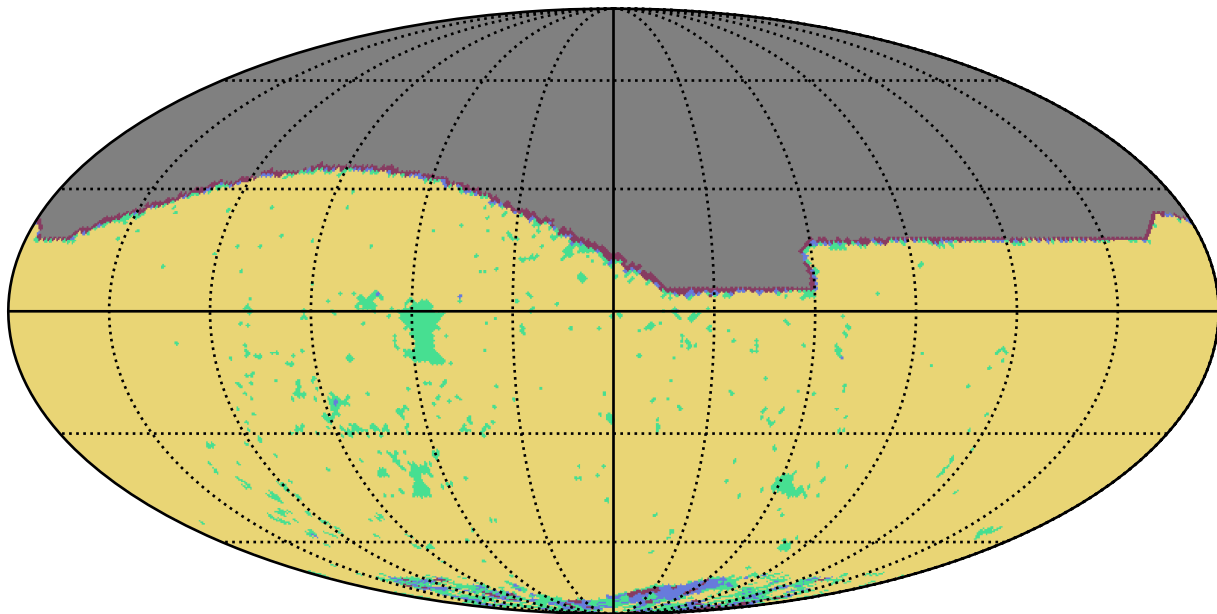
too_5_1v3.4_10yrs i band: YearCoverage night
