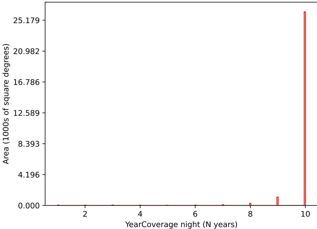
too_5_1v3.4_10yrs i band: YearCoverage night
