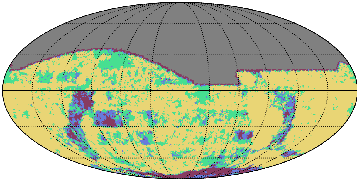
too_5_1v3.4_10yrs g band: YearCoverage night
