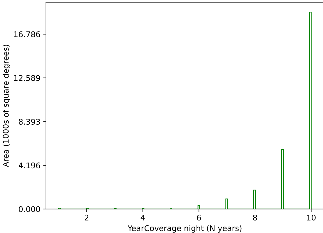
too_5_1v3.4_10yrs g band: YearCoverage night
