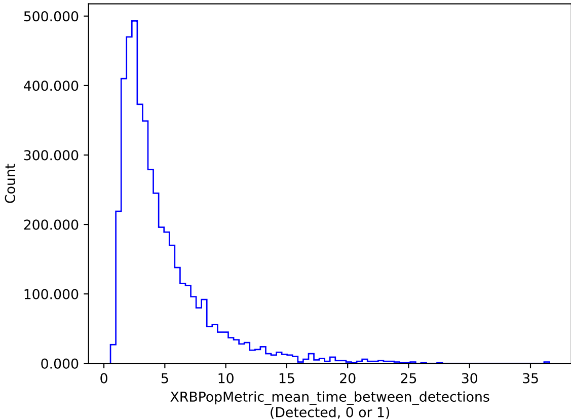
too_5_1v3.4_10yrs : XRBPoMetric_mean_time_between_detections
