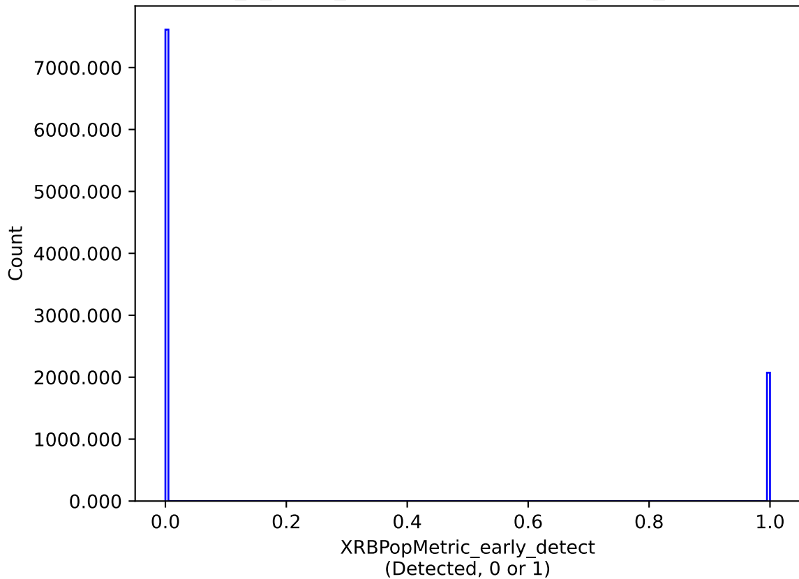
too_5_1v3.4_10yrs : XRBPoMetric_early_detect
