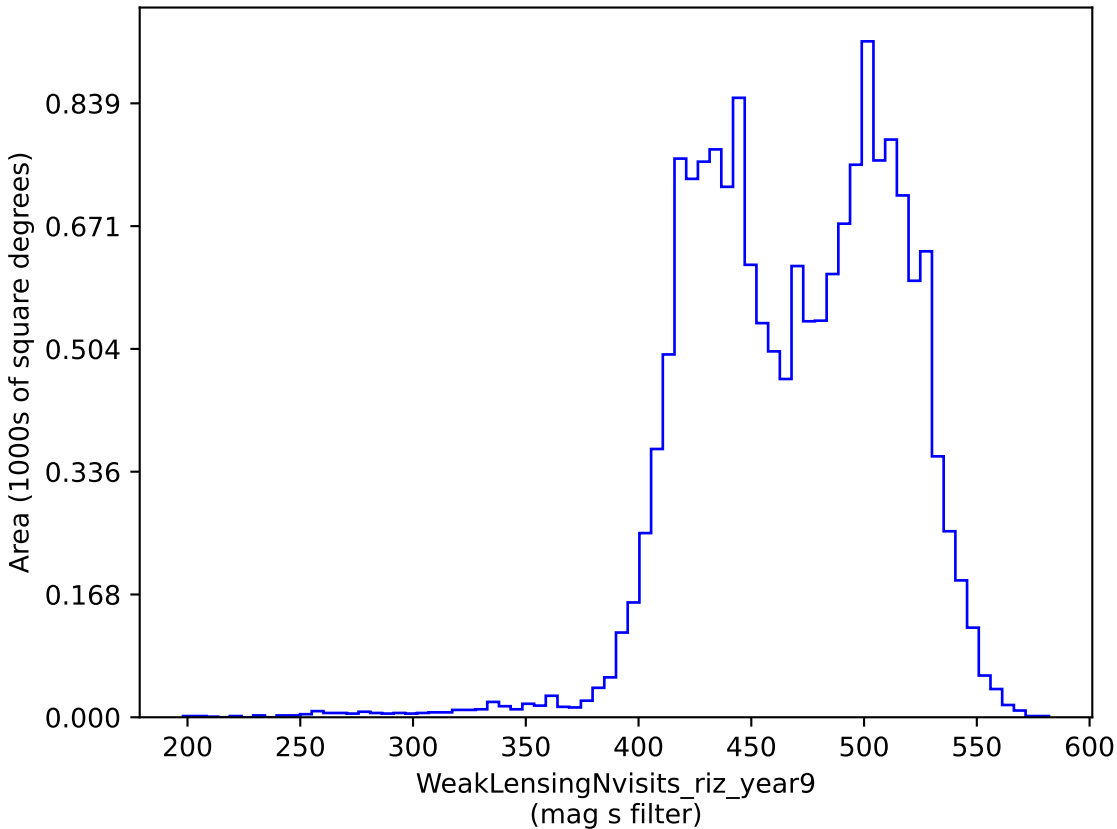
too_5_1v3.4_10yrs gri band non-DD: WeakLensingNvisits_riz_year9
