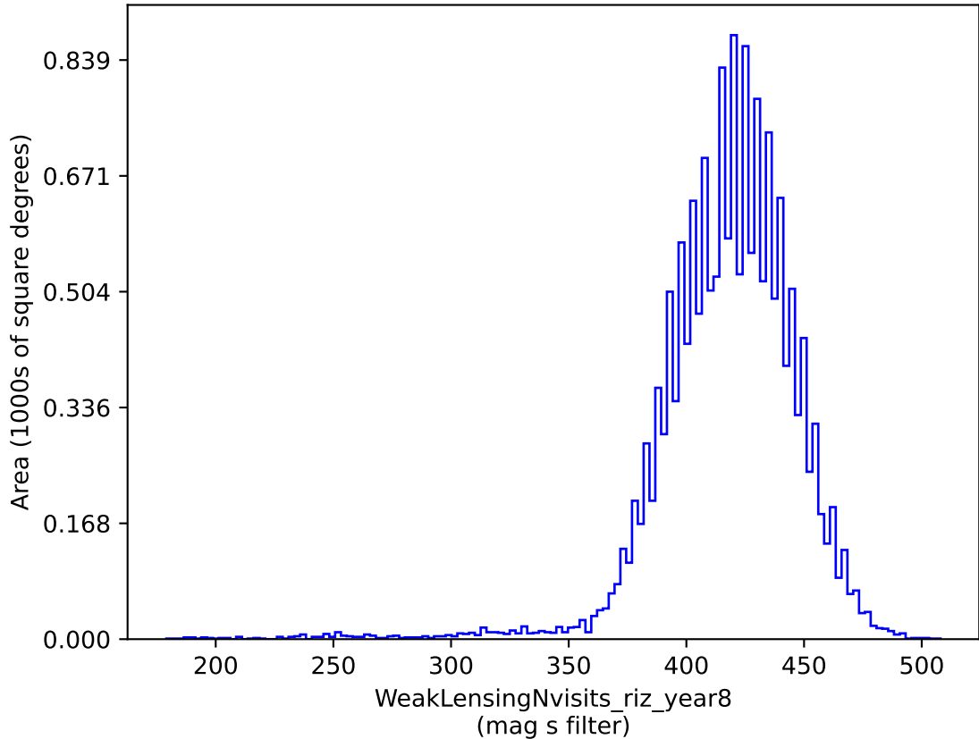
too_5_1v3.4_10yrs gri band non-DD: WeakLensingNvisits_riz_year8
