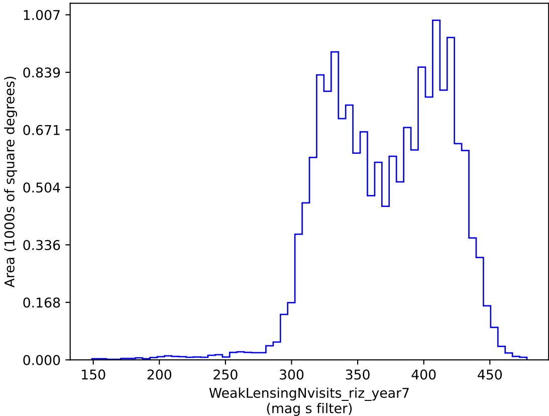
too_5_1v3.4_10yrs gri band non-DD: WeakLensingNvisits_riz_year7
