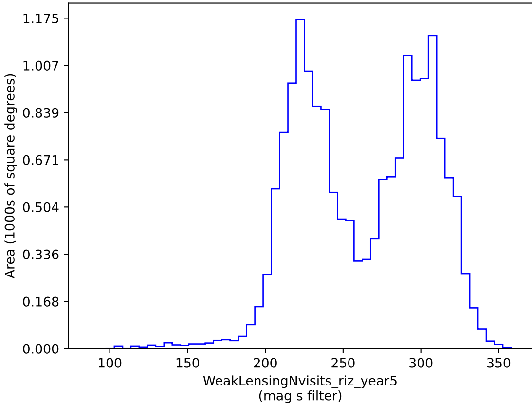
too_5_1v3.4_10yrs gri band non-DD: WeakLensingNvisits_riz_year5
