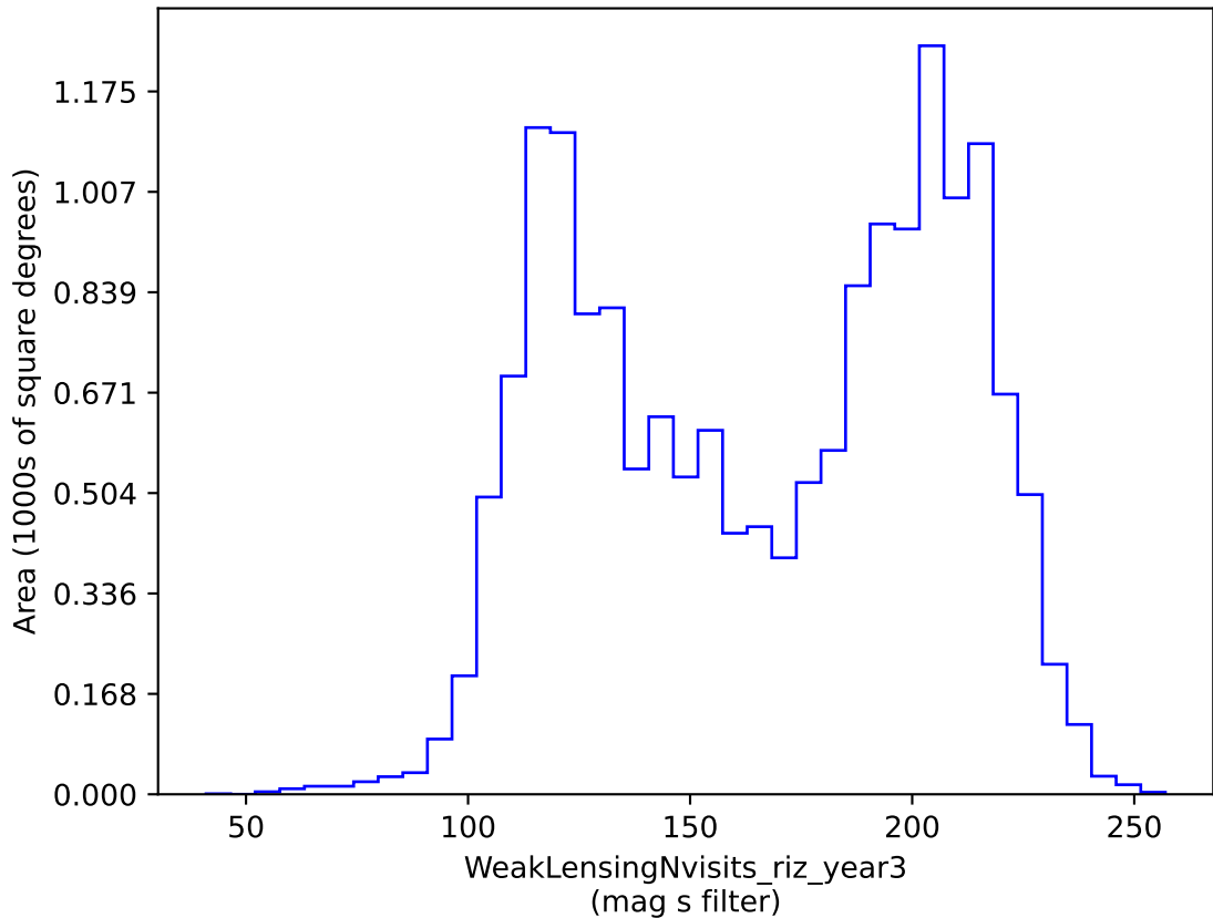
too_5_1v3.4_10yrs gri band non-DD: WeakLensingNvisits_riz_year3
