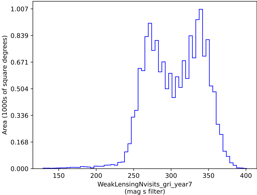
too_5_1v3.4_10yrs gri band non-DD: WeakLensingNvisits_gri_year7
