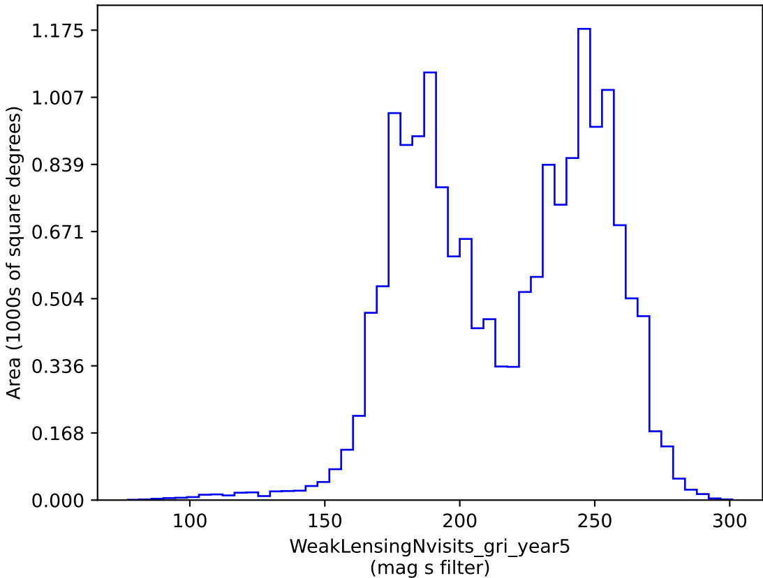
too_5_1v3.4_10yrs gri band non-DD: WeakLensingNvisits_gri_year5
