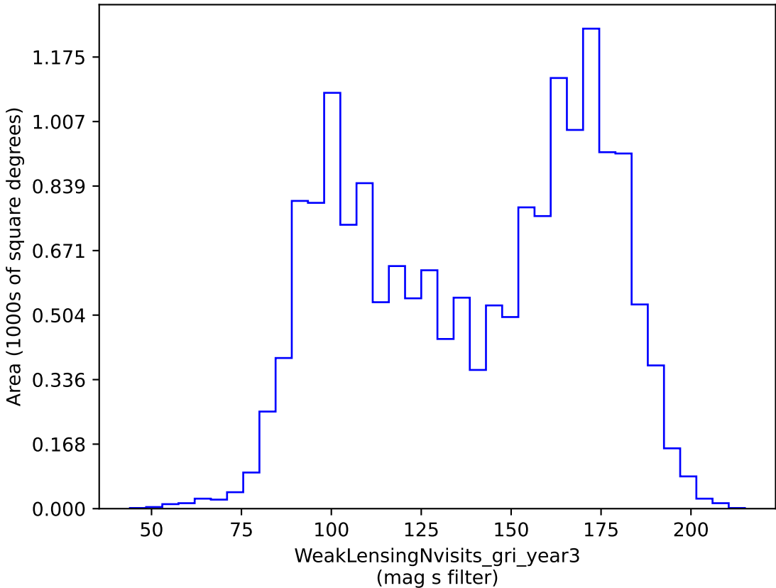
too_5_1v3.4_10yrs gri band non-DD: WeakLensingNvisits_gri_year3
