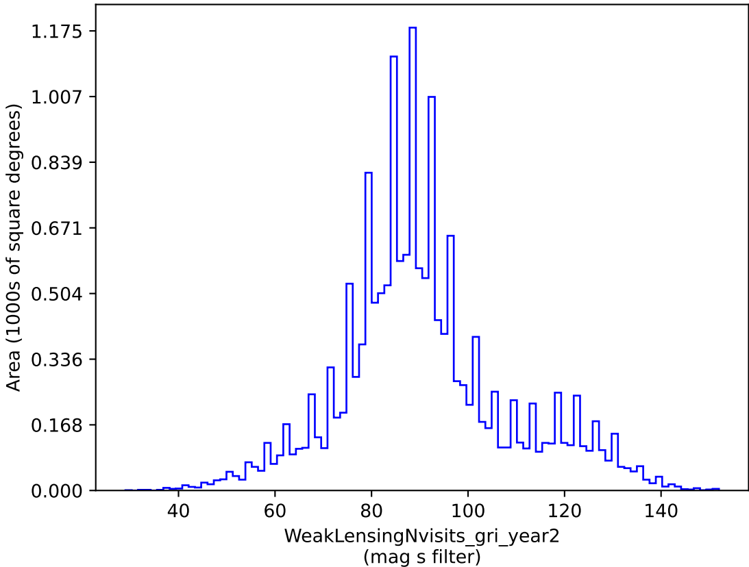
too_5_1v3.4_10yrs gri band non-DD: WeakLensingNvisits_gri_year2
