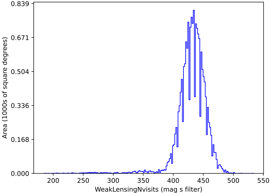
too_5_1v3.4_10yrs gri band non-DD: WeakLensingNvisits
