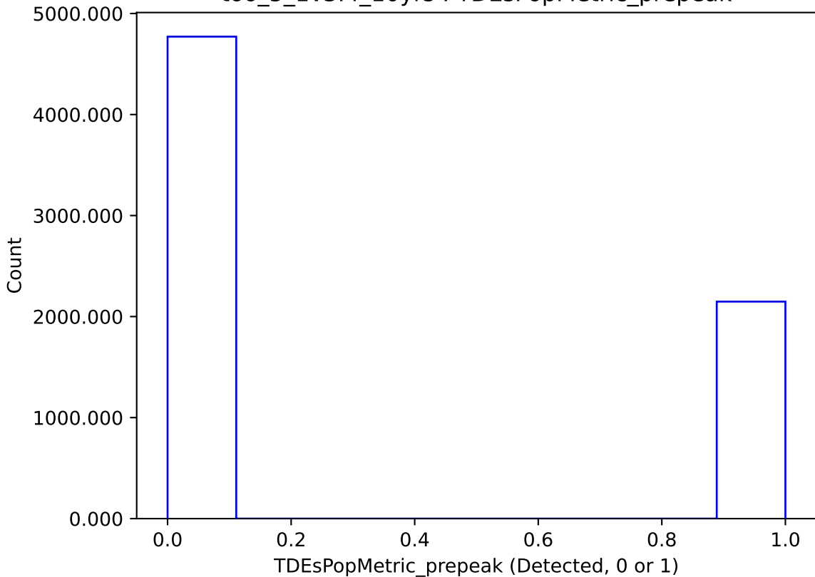
too_5_1v3.4_10yrs : TDEsPopMetric_prepeak
