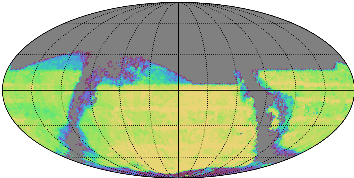
too_5_1v3.4_10yrs : TDC_season
