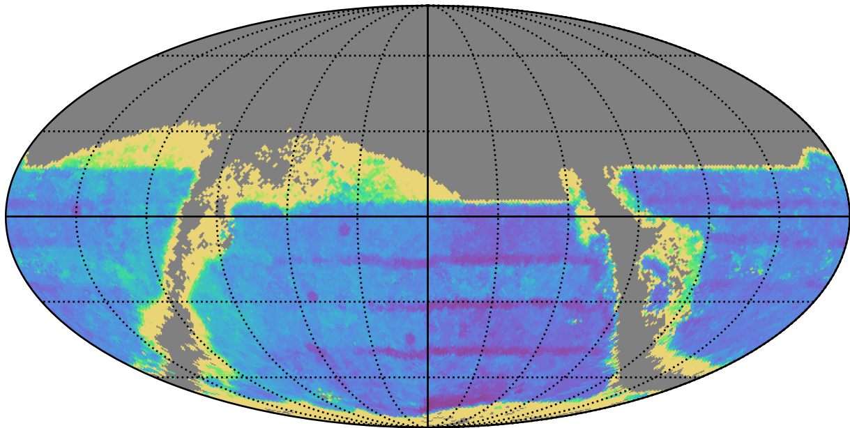
too_5_1v3.4_10yrs : TDC_accuracy
