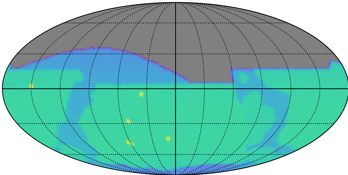
too_5_1v3.4_10yrs z: SurfaceBrightLimit
