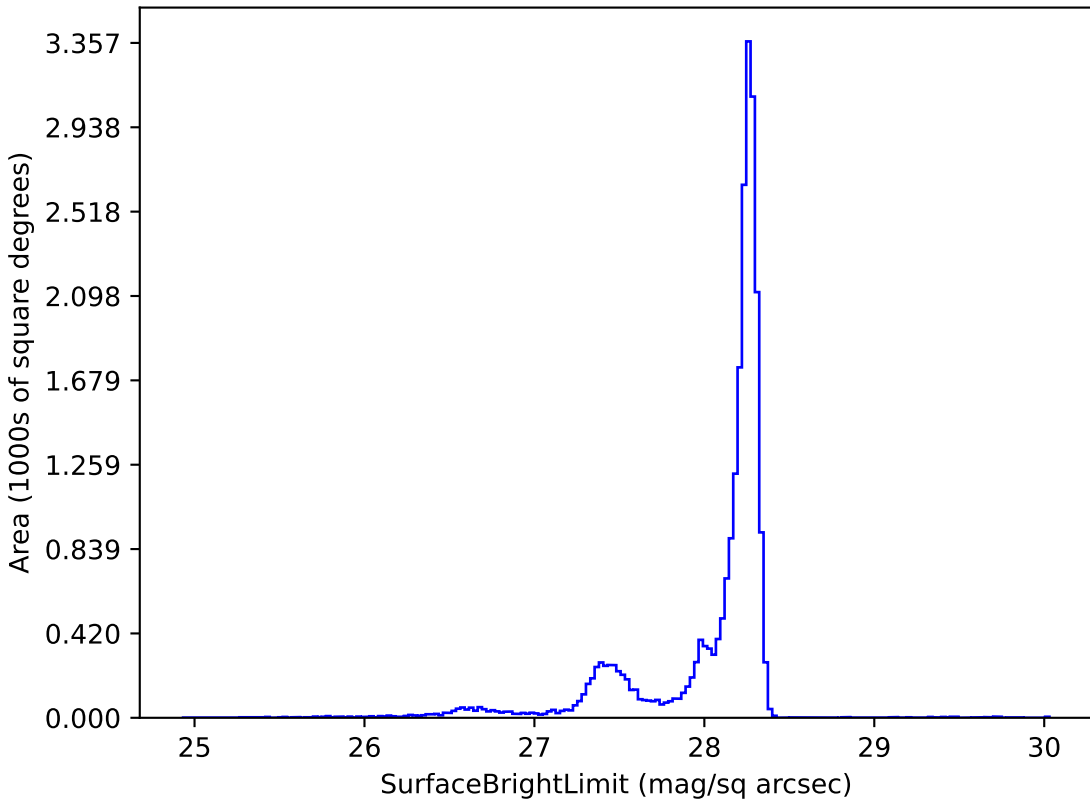
too_5_1v3.4_10yrs y: SurfaceBrightLimit
