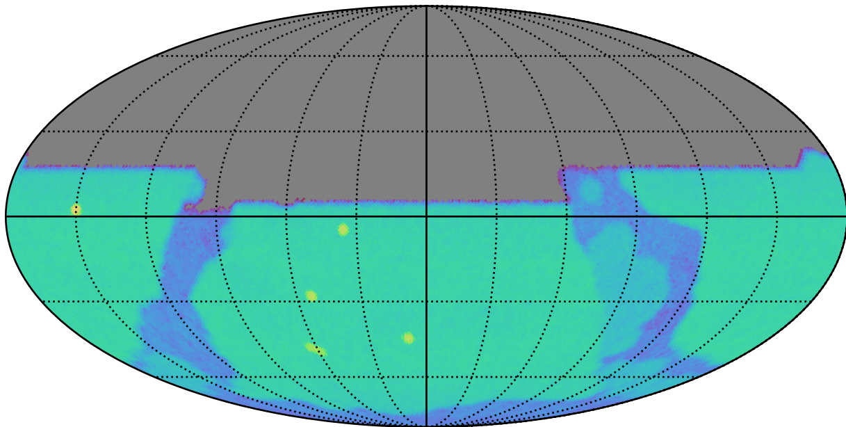
too_5_1v3.4_10yrs u: SurfaceBrightLimit
