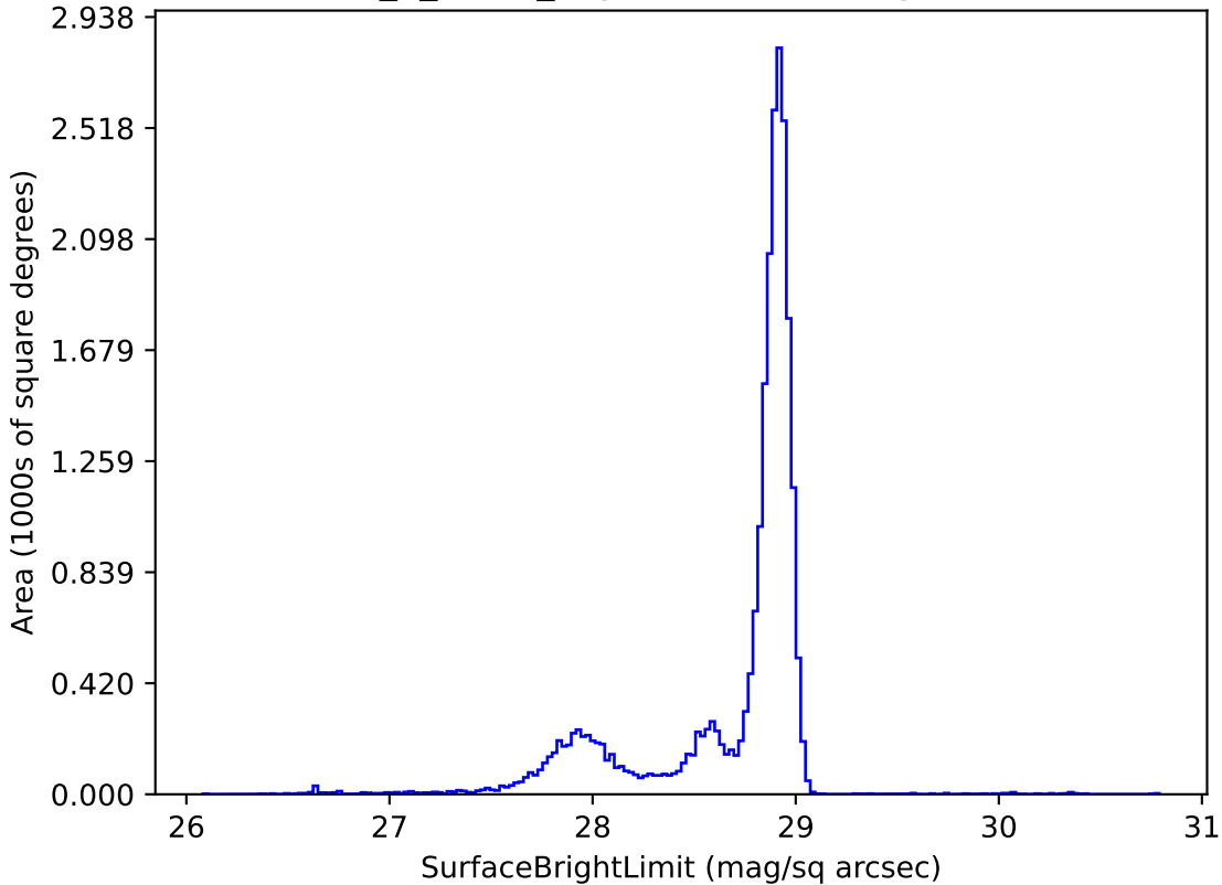
too_5_1v3.4_10yrs u: SurfaceBrightLimit
