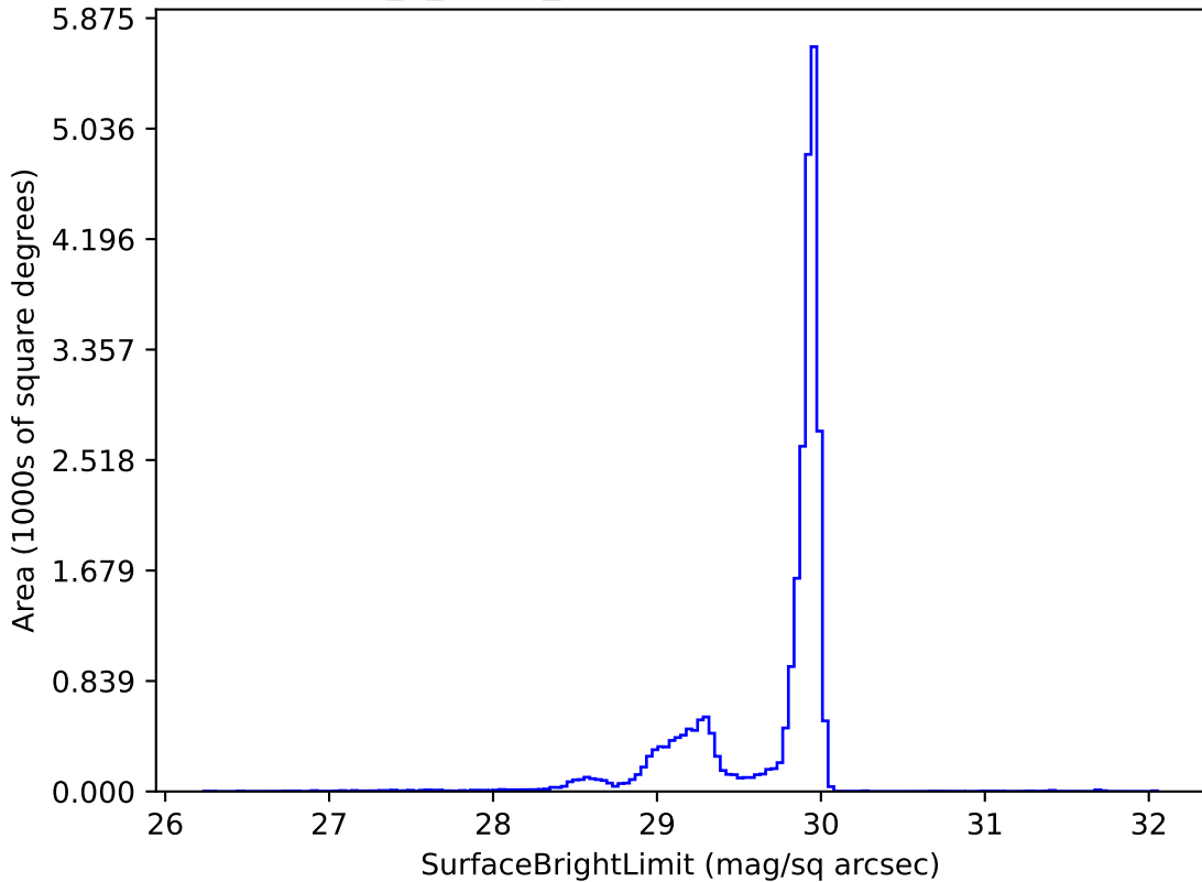
too_5_1v3.4_10yrs i: SurfaceBrightLimit
