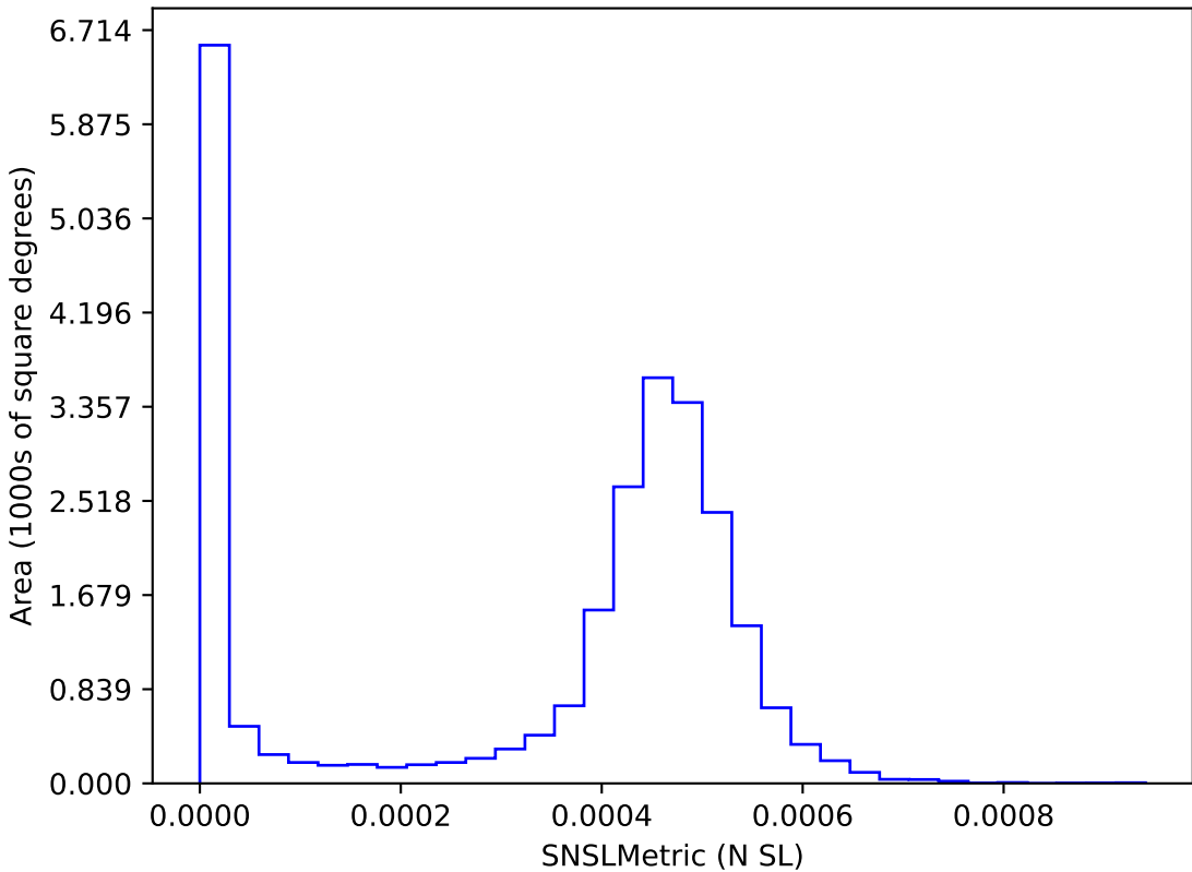
too_5_1v3.4_10yrs : SNSLMetric
