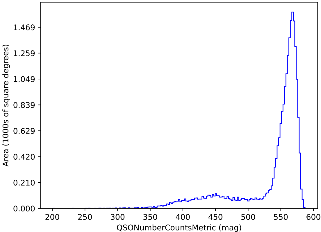
too_5_1v3.4_10yrs y band and non-DD: QSONumberCountsMetric
