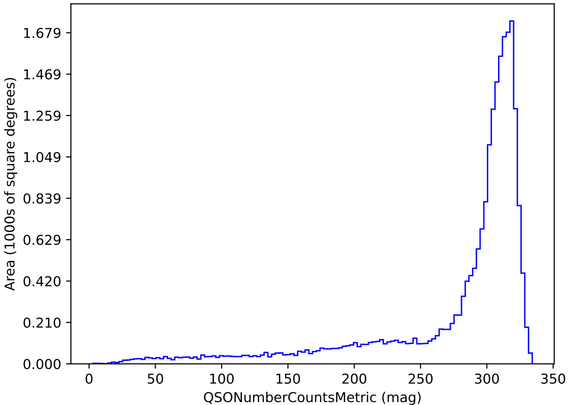
too_5_1v3.4_10yrs u band and non-DD: QSONumberCountsMetric
