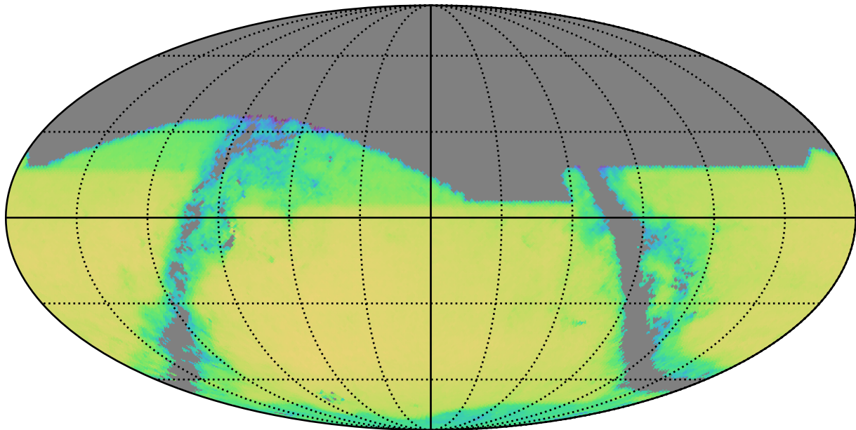
too_5_1v3.4_10yrs r band and non-DD: QSONumberCountsMetric
