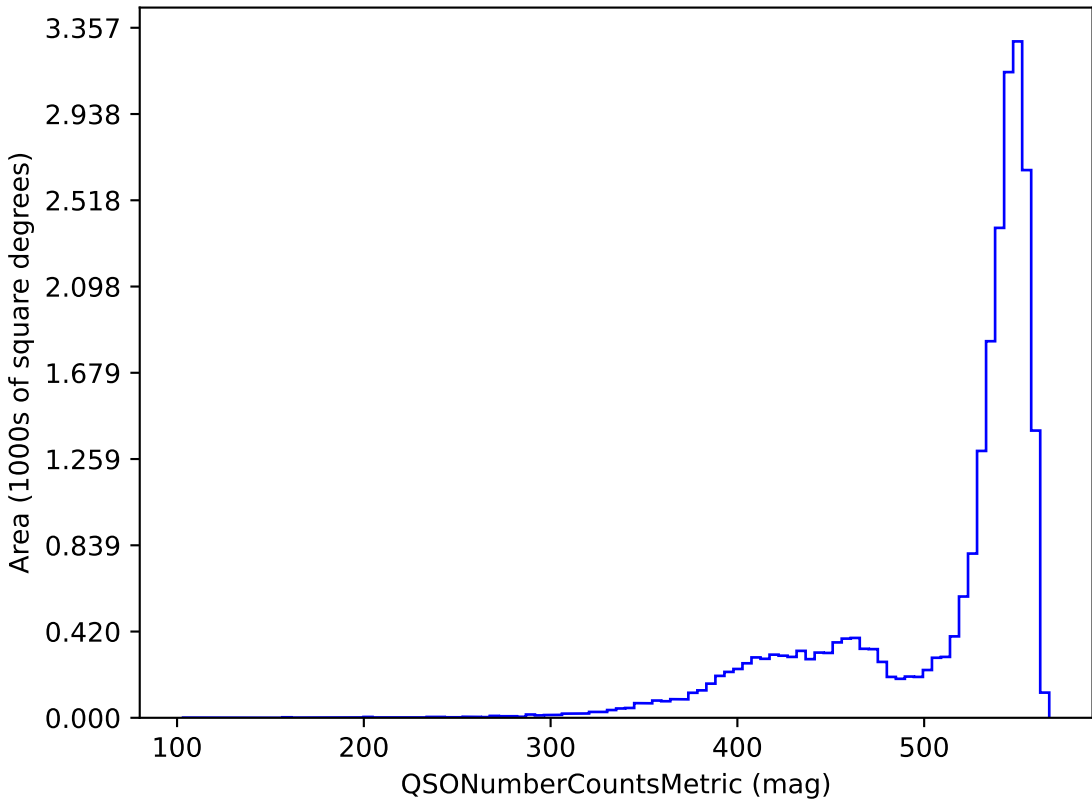
too_5_1v3.4_10yrs i band and non-DD: QSONumberCountsMetric
