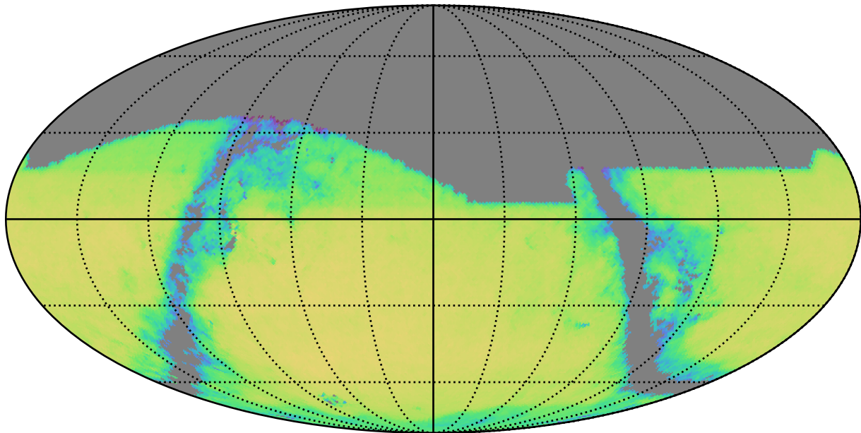
too_5_1v3.4_10yrs g band and non-DD: QSONumberCountsMetric
