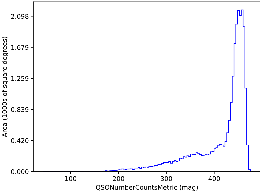
too_5_1v3.4_10yrs g band and non-DD: QSONumberCountsMetric
