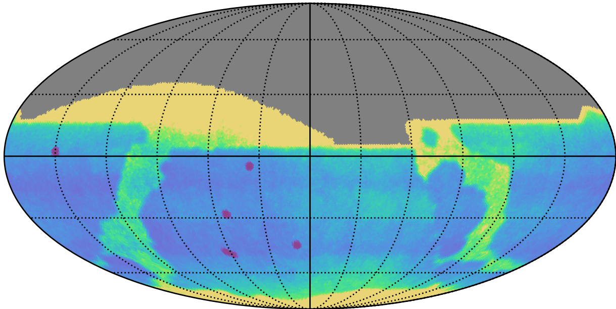
too_5_1v3.4_10yrs : Proper Motion Uncert @ 24.0
