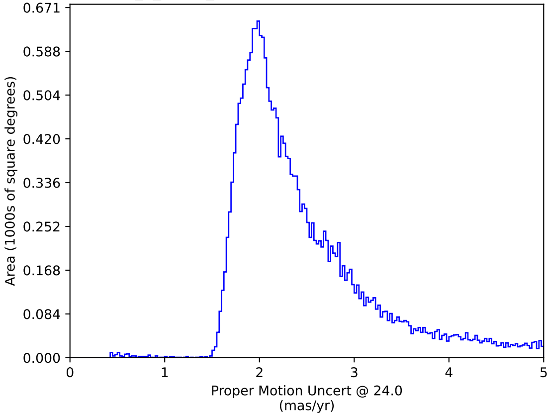
too_5_1v3.4_10yrs : Proper Motion Uncert @ 24.0
